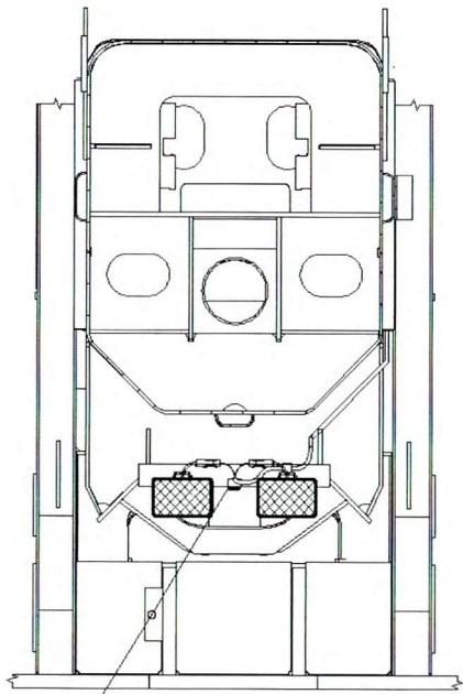
SECTION A-A BOOM LIGHTS SEE VIEW AA LMI ALARM
